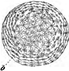
FIG. 73.—Gemmule of E. fluviatilis . b , Amphidisc. (After Potts.)
